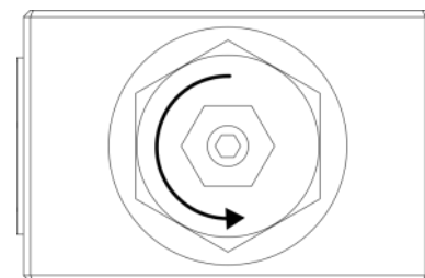
End View, Flow Divider Turn Counter-clockwise to loosen nut and set screw.
