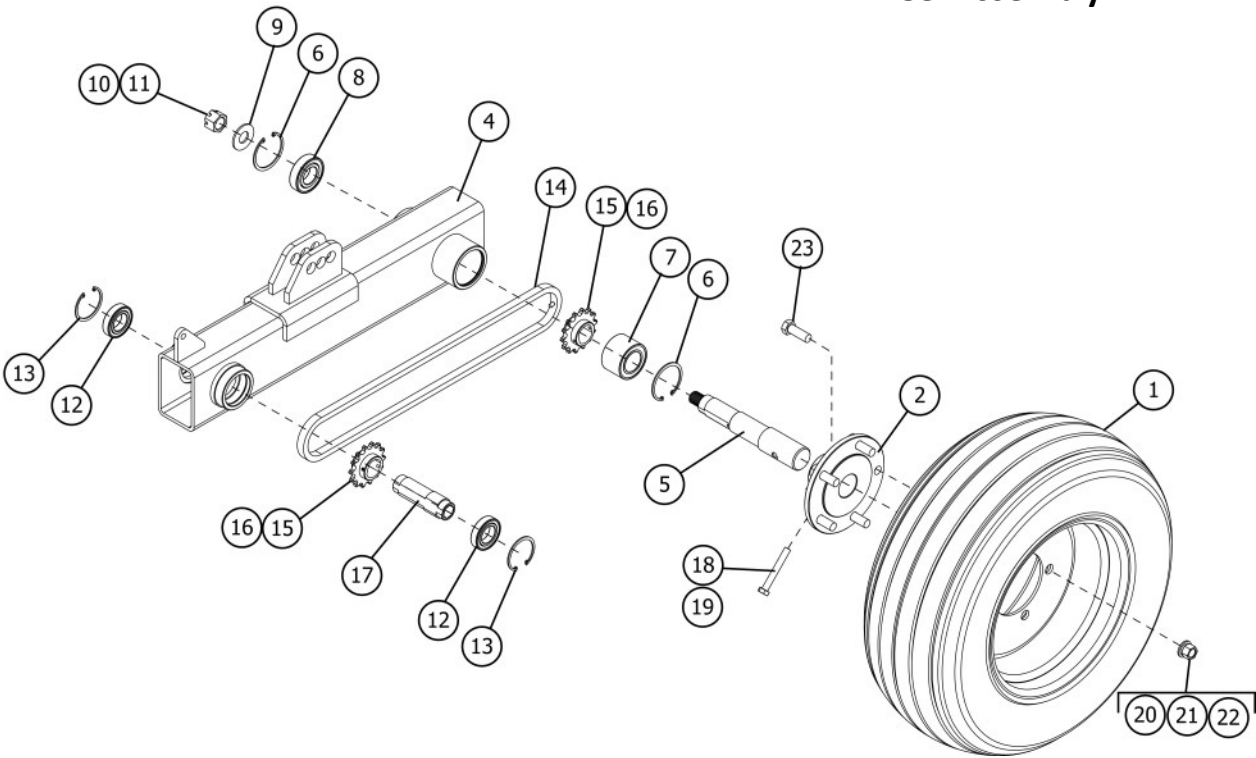
LH Wheel Assembly
